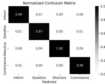
Fig. 2. Normalized confusion matrix for Stage 1 dialogue act classification (4-class: Inform, Question, Directive, Commissive).
