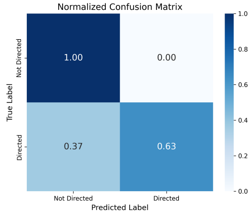
Fig. 3. Normalized confusion matrix for Stage 2 binary directedness classification (Directed vs. Not Directed).
